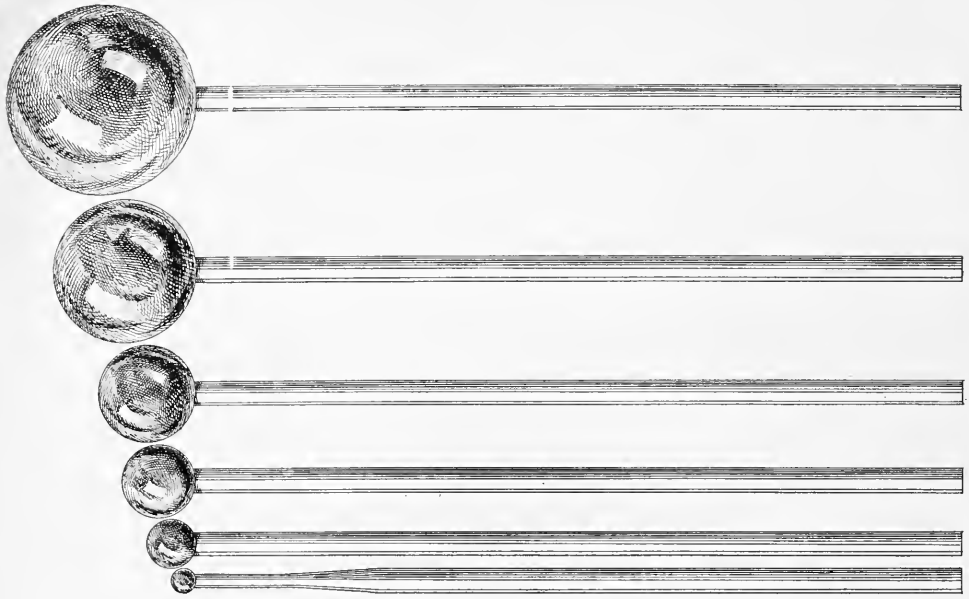
FIG. 51.—Glass balls to which handles are attached, for measuring orifices. (Actual size.)
